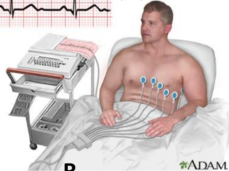
Electrocardiogram (ECG)
